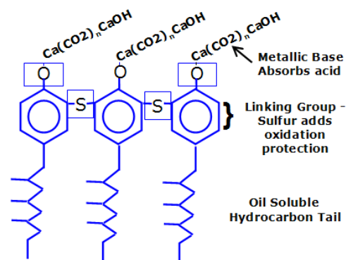
Figure 1. The chemical structure of a phenate contains four critical parts. 1) Hydrocarbon tail, 2) Linking group, 3) Metallic carbonate, 4) Sulfur
